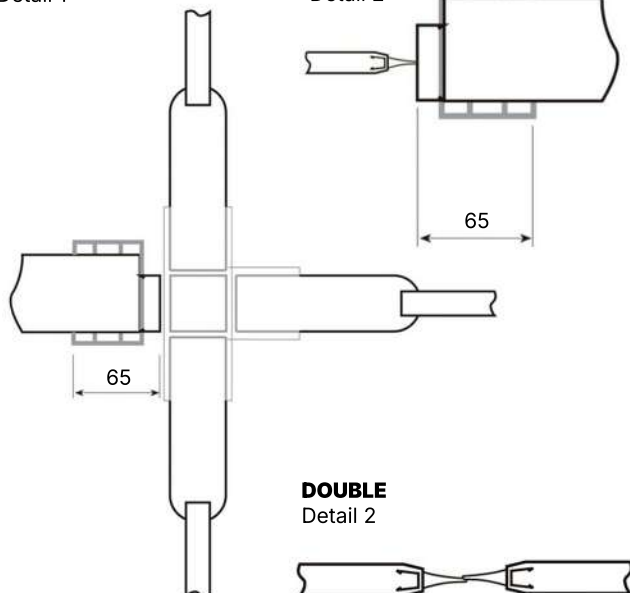
SIMPLE / DOUBLE Detail 1
