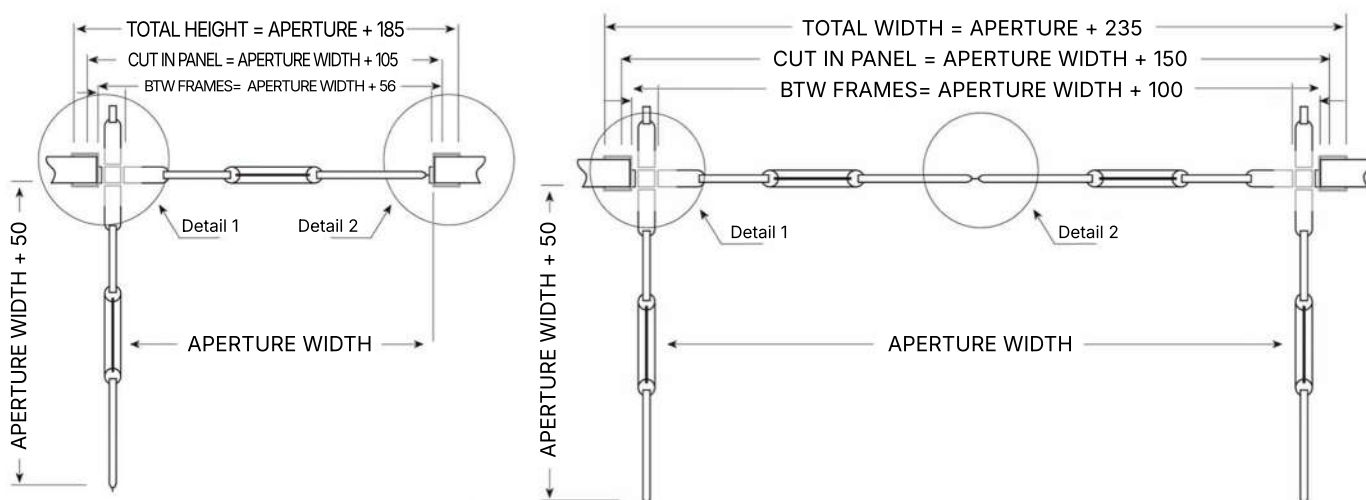
SIMPLE / DOUBLE Detail 1
