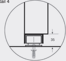
SINGLE / DOUBLE Detail 4
